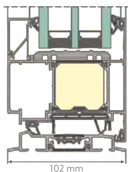
CROSS SECTION OF DOOR THRESHOLD
